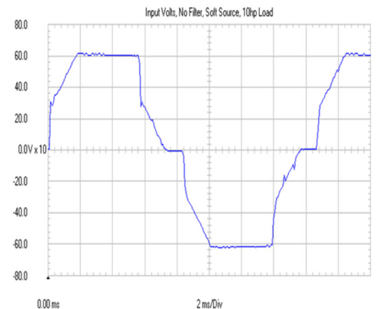
LINE VOLTAGE, NO FILTER Fig. 7 THVD = 13.8%
