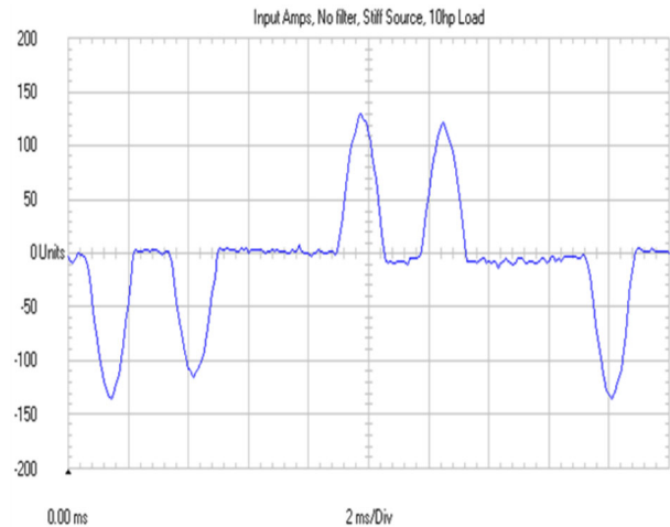
LINE CURRENT, NO FILTER Fig. 1 THID = 108%
