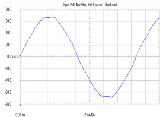
LINE VOLTAGE, NO FILTER Fig. 3 THVD = 2.2%
