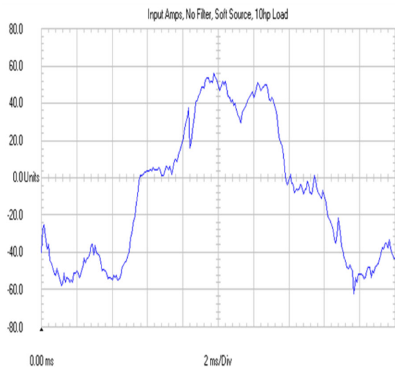
LINE CURRENT, NO FILTER Fig. 5 THID = 25.8%
