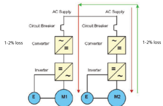
Figure 8 Standalone drives
